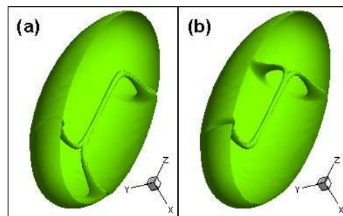
FIG. 4: Comparison between the single vortex configurations obtained for the same angular velocity \Omega/\omega_x = 0.44 . Superposition of the U and S vortex (a) and the planar and non-planar S vortex (b).
